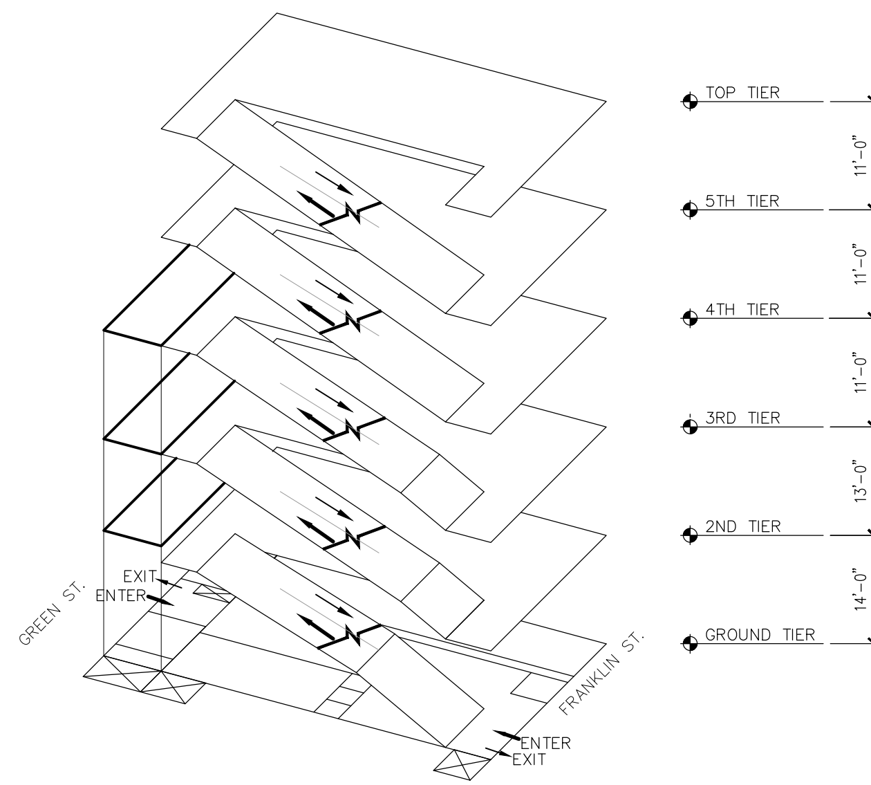
ISOMETRIC
